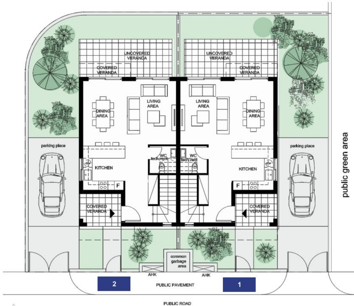
GROUND FLOOR
