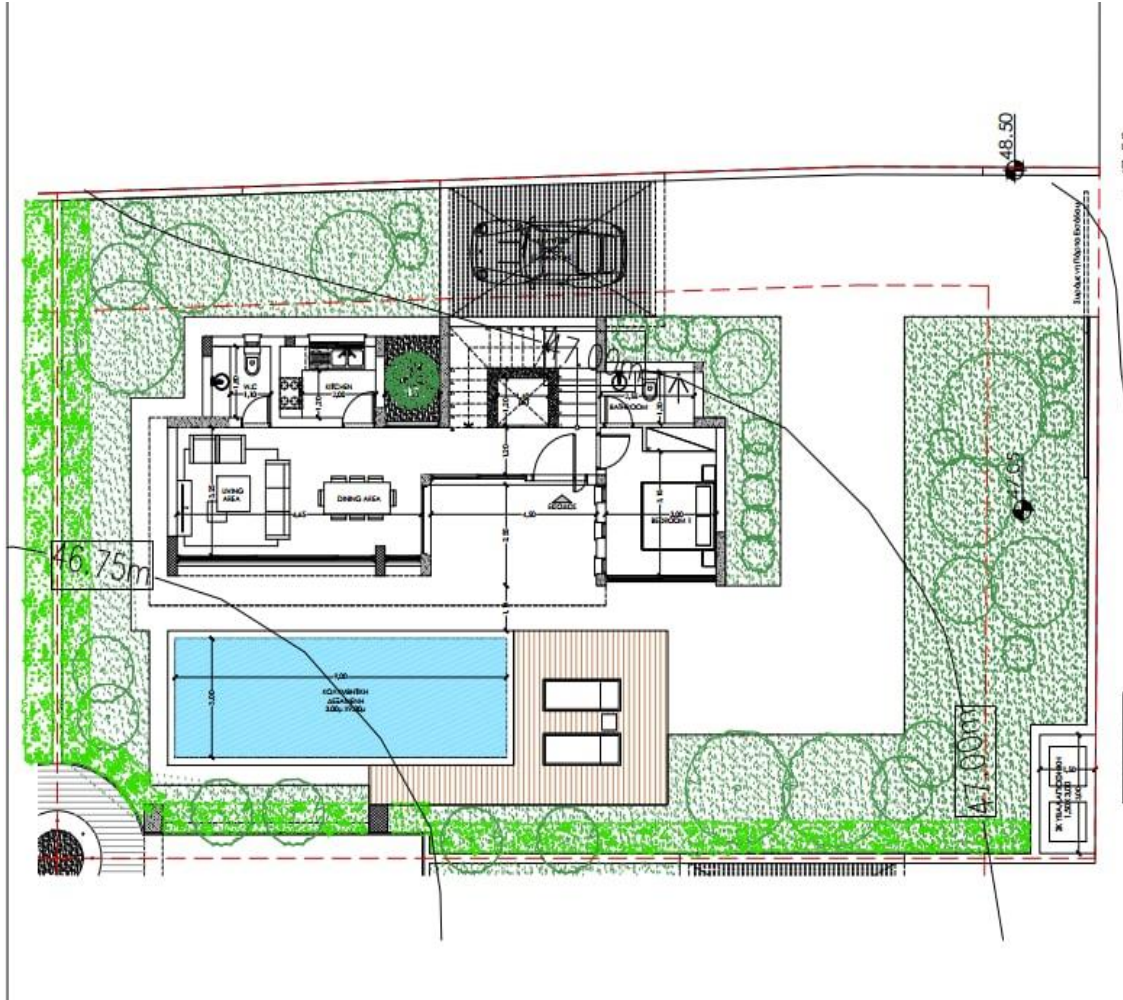
GROUND FLOOR
