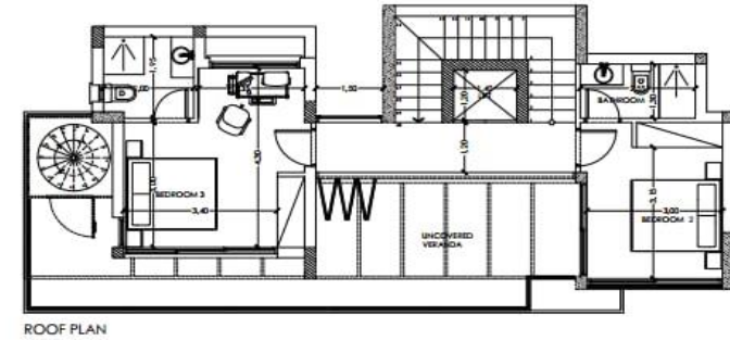
ROOF PLAN
